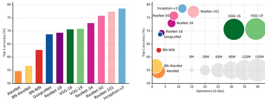
Figure 3..Comparison of Inception V3 with other CNN models
