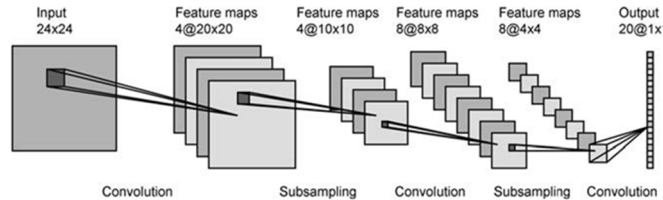
Figure 4. Working of convolutional network
